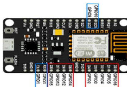
Figure 2: NodeMCU
