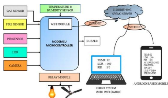
Figure 1: Block diagram of IoT based Smart Home Automation and Scrutiny System
