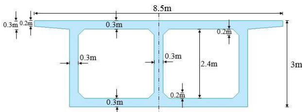
Fig.2: Two-cell rectangular box girder (TCR)
