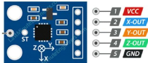
Fig.3: ADXL335 accelerometer
