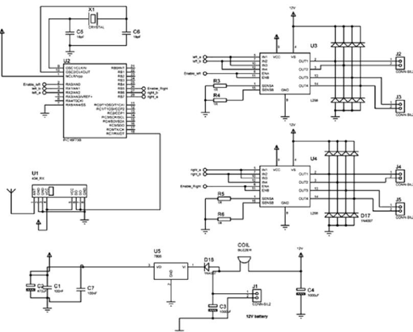
Fig.9: (b) Transmitter Circuit
