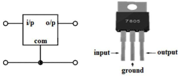
Fig.8: Voltage Regulator
