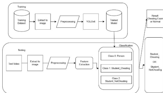
Figure 1: Validation and testing
