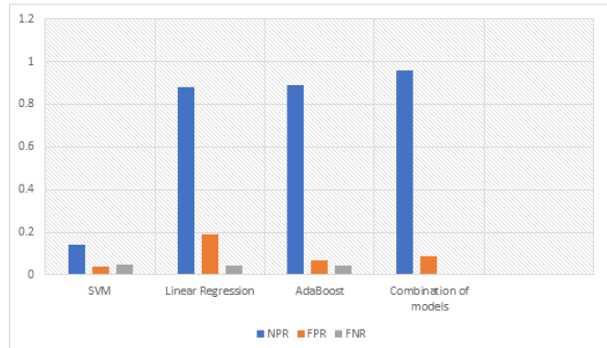
Figure 5: Positive and negative rate prediction
