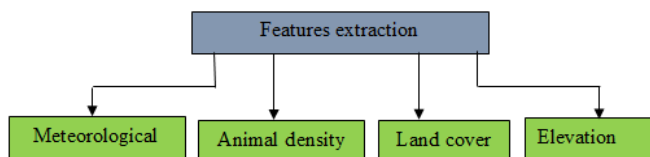
Figure 2: Feature extraction
