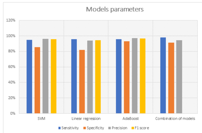
Figure 4: Model evaluation parameters
