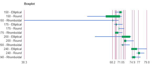
Figure 7: Box Plot
