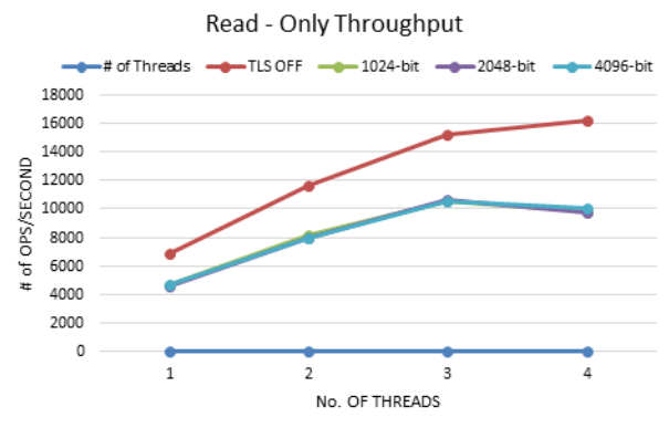
Figure 3: TLS Read-only throughput Overhead on Mongo DB
