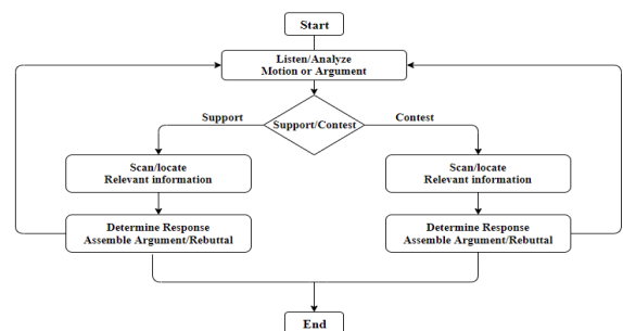
Figure 4: Activity diagram of AI debater system
