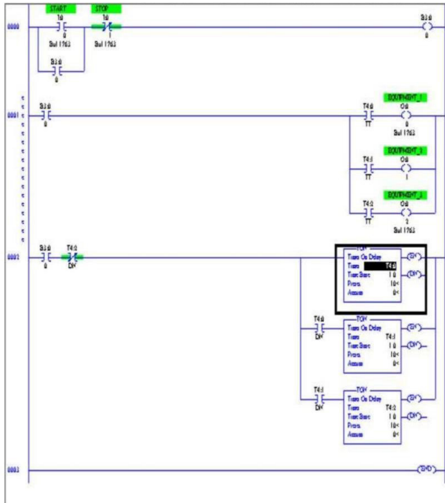
Fig. 1: Ladder Diagram
