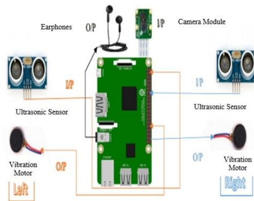
Figure 2: Hardware Configuration of the Device
