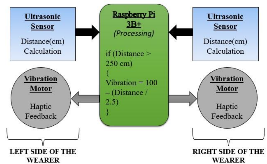
Figure 3: Block Diagram for Navigation
