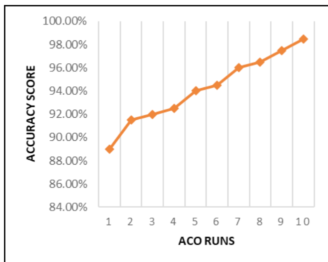
Figure 6: Graphical Representation of accuracy using NB Algorithm
