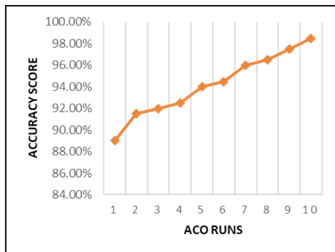
Figure 8: Graphical representation of accuracy using LR algorithm
