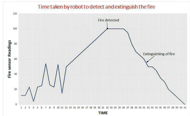
Figure 17: Graph showing fire sensor readings vs. time (seconds) taken by the robot to detect and extinguish fire
