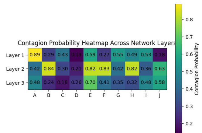
Fig 6: Heatmap displays estimated contagion probabilities across three interconnected network layers, with higher color intensity indicating elevated systemic spillover risk. Overlaid values provide precise probability estimates for each bank-layer interaction.
