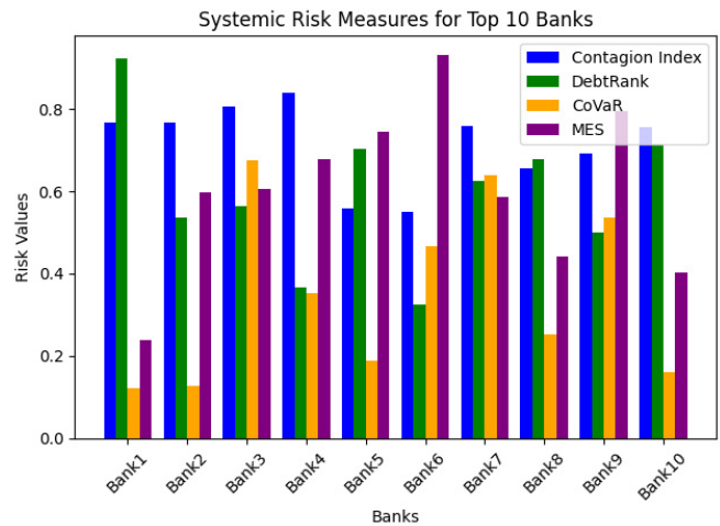
Fig 2: Comparative bar chart of Contagion Index, DebtRank, CoVaR, and MES for the top ten systemically important banks. Values are simulated for illustrative purposes to demonstrate cross-metric variation in systemic risk profiles.
