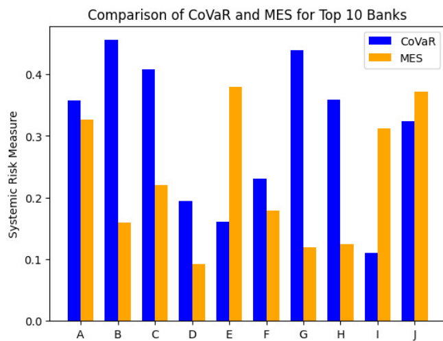
Fig 5: Bars compare CoVaR (Conditional Value at Risk) and MES (Marginal Expected Shortfall) across the top 10 banks, illustrating methodological differences in systemic risk contribution and tail-risk sensitivity.
