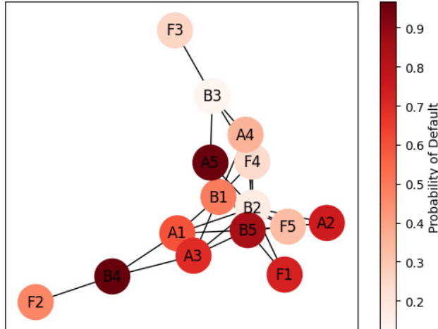
Cascading Failure in Multi-Layer Financial Network
