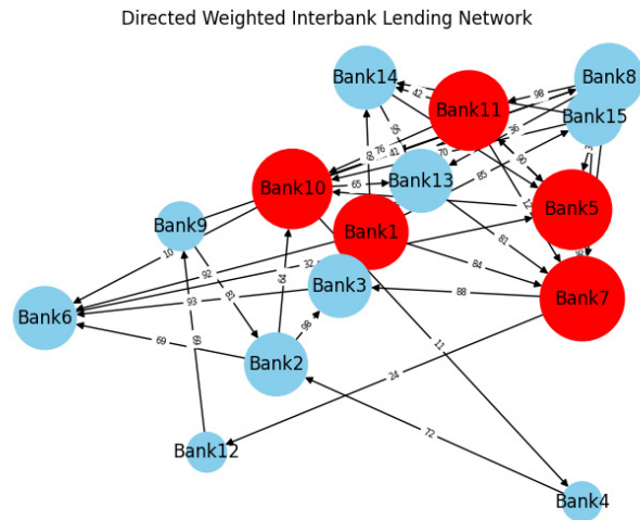
Fig 1: Directed and weighted interbank exposure network. Node size reflects degree centrality as a proxy for systemic importance, edge weights denote bilateral credit exposures, and the top five systemically important banks are highlighted in red.
